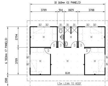
Shared Accommodation Unit 4 bedroom, 2 showers, toilet and veranda 66.1m 2
