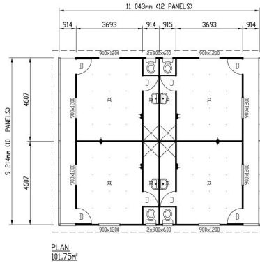
Skilled Workers Accommodation Unit 4 bedroom en suite 101.75m 2
